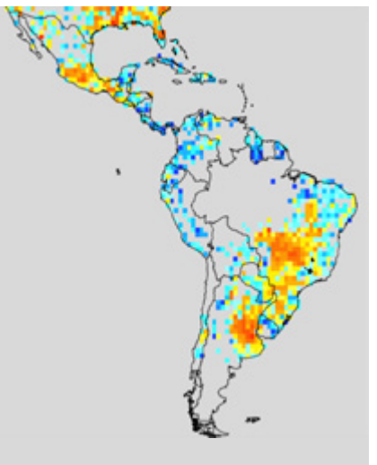
SLCP mitigation + climate vs. reference
