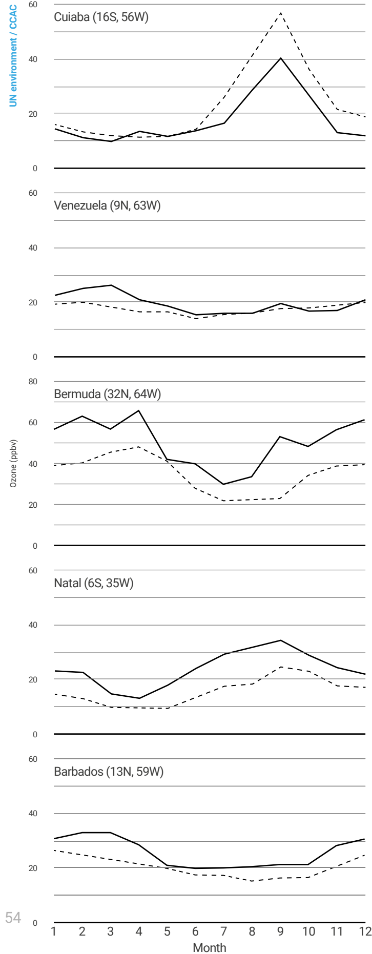
Figure 1.16 Comparison of GISS model monthly mean surface ozone values (solid line) with observations at selected stations in Latin America and the Caribbean Source: Logan, 1999; Thompson et al. , 2007. With O 3 , a comparison of the GISS estimates with monitoring reveals similar patterns of O 3 concentrations over the year (Figure 1.16), though at particular stations the model estimates may be higher or lower than the monitored values.
