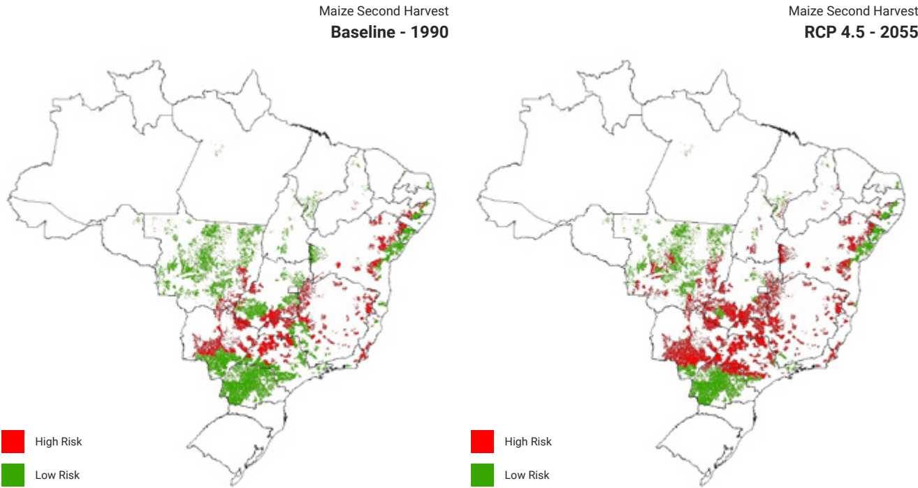
Figure A Impact of global warming on second maize harvest in Brazil, baseline 1990
