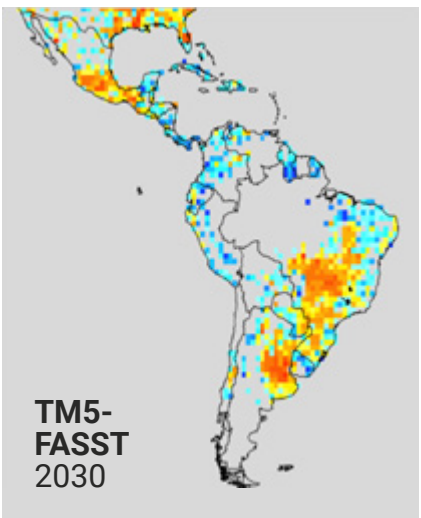
SLCP Mitigation vs. reference
