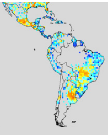
Climate vs. reference
